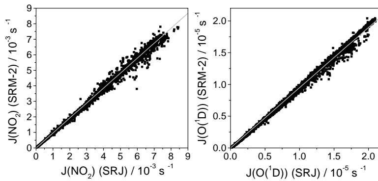
Fig. 8. Correlation plot of J(O(^1D)) and J(NO_2) of the SRM (SRM-2) against SRJ for all measured data in the period 21 May 1999–28 May 1999.
