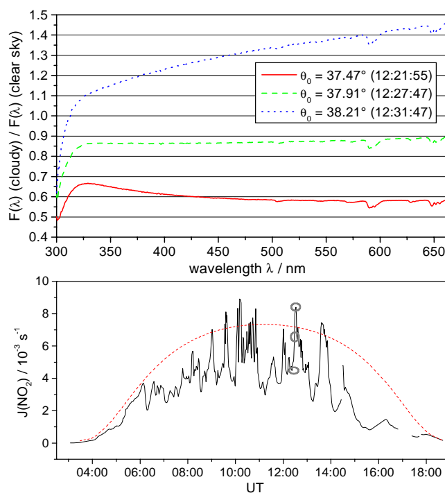
Fig. 11. Deviation of spectra measured during partial cloud cover in relation to clear-sky spectra. The times of the chosen spectra are marked in the photolysis frequency J(NO_2) in the lower panel. The dashed line in the lower panel is the parameterized clear sky J(NO_2) . In the upper panel, the dotted line corresponds to a point at a local maximum above the clear sky value, the dashed line corresponds to a point near the clear-sky case and the full line corresponds to a local minimum value.
