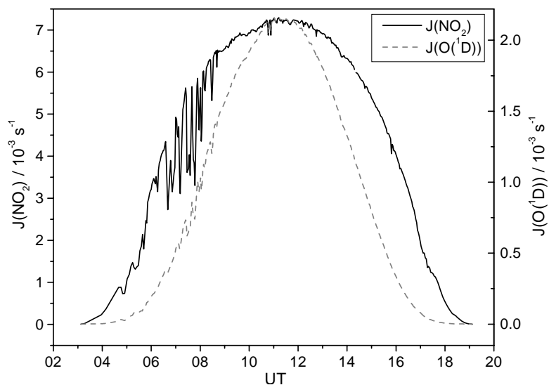
Fig. 10. Photolysis frequencies J(O(^1D)) and J(NO_2) measured with the SRM on 9 August 1998 during the field campaign BERLIOZ in Berlin on the roof of the Charité building. Partial cloud cover in the time from 05:00 to 09:00 UT leads to reductions and enhancements in the photolysis frequencies, whereas the effect is more pronounced in J(NO_2) .
