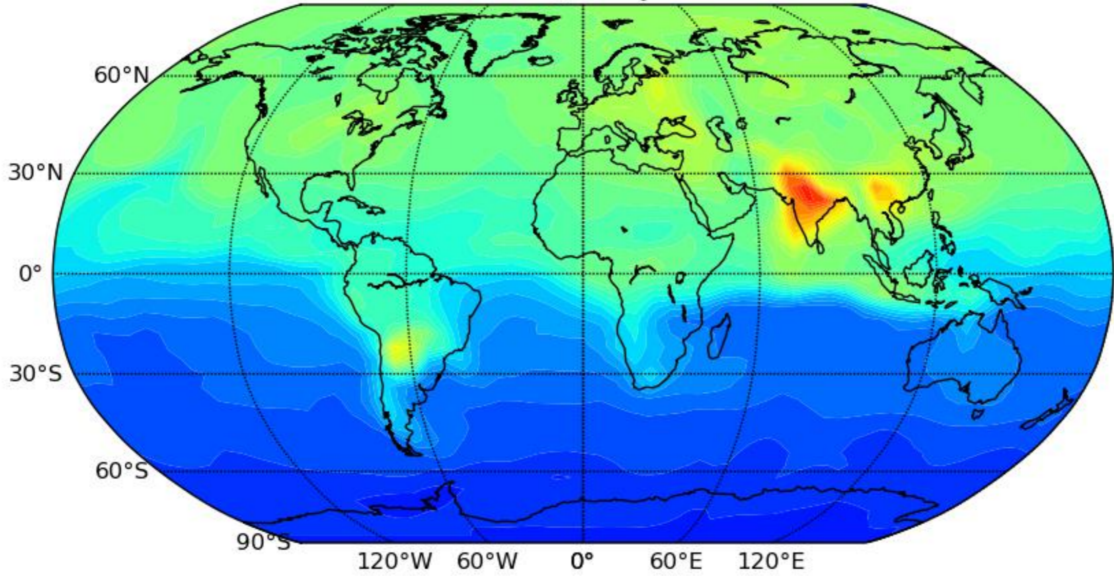
Column Average CH 4 20101231
